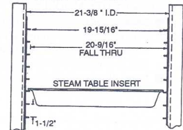
ALUMINUM EXTRUDED SIDE PANEL
