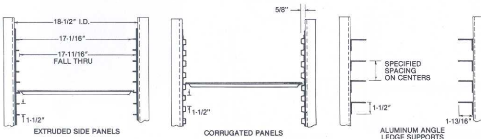
Model 9220-39-PT Extruded Sides Pass Thru' Cabinet
