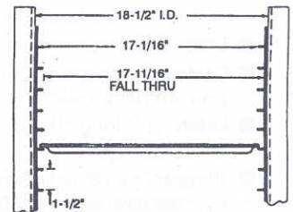
ALUMINUM EXTRUDED SIDE PANEL
