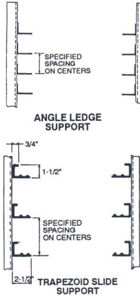
Trapezoid Slide Type Model 9170-1824 (Double side loading)
